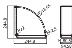
KOLJENO CRO 90 220X90 MM FUN 112.0459.455
