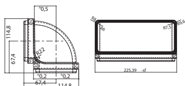
KOLJENO CRV 90 220X90 MM FUN 112.0459.453
