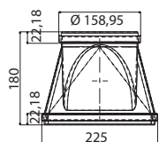
SPOJNICA RRC 220X90 MM FUN 112.0459.429
