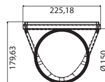
KOLJENO CRC 90 220X90 MM FUN 112.0459.451
