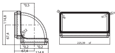
NOSAČ FRF 220X90 MM FUN 112.0459.456
