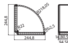
KOLJENO CRO 90 220X90 MM FUN 112.0459.455
