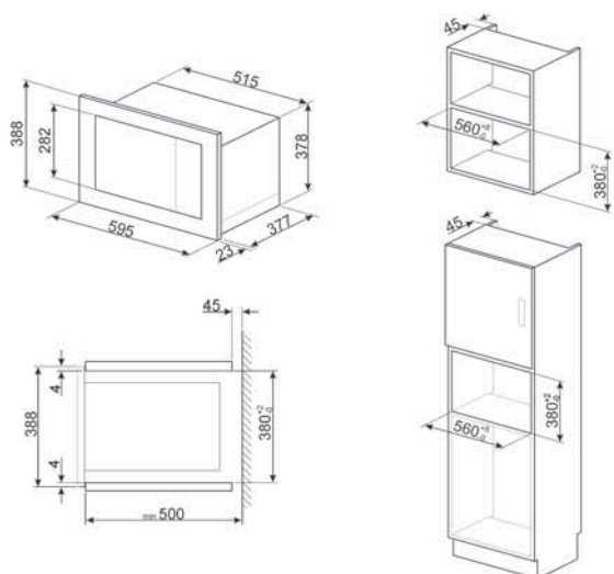
MIKROVALNE PEČNICE: FMI625CTI, FMI125G, FMI125N, FMI425X
